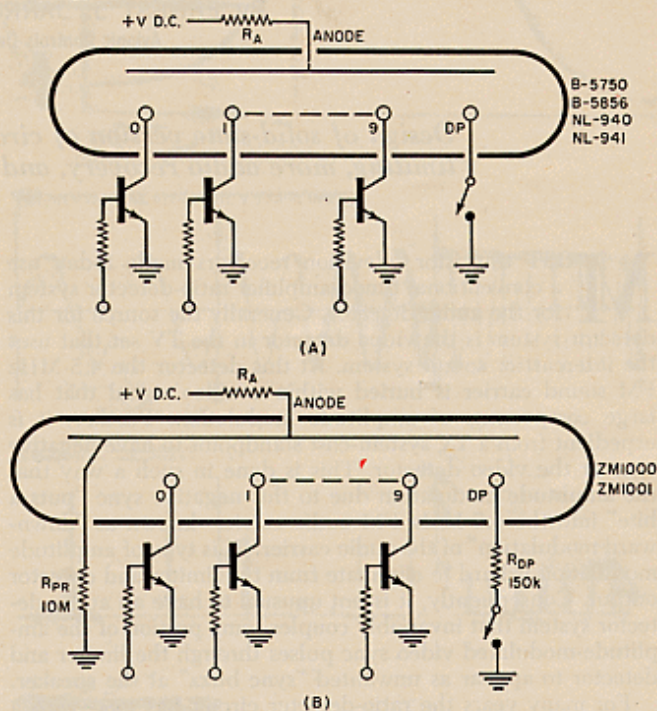
Fig. 6. Driver circuit configurations for (A) Burroughs B-5750 and B-5856 and National's NL-940 and NL-941 devices that do not require separate decimal-point resistor unless the decimal point is energized alone and for (B) Amprex Types ZM1000 and ZM1001 which require a priming resistor. Type ZM1000 also requires separate decimal-point resistor.
